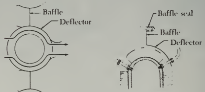
FIGURE 6-34. Heat dissipation.
